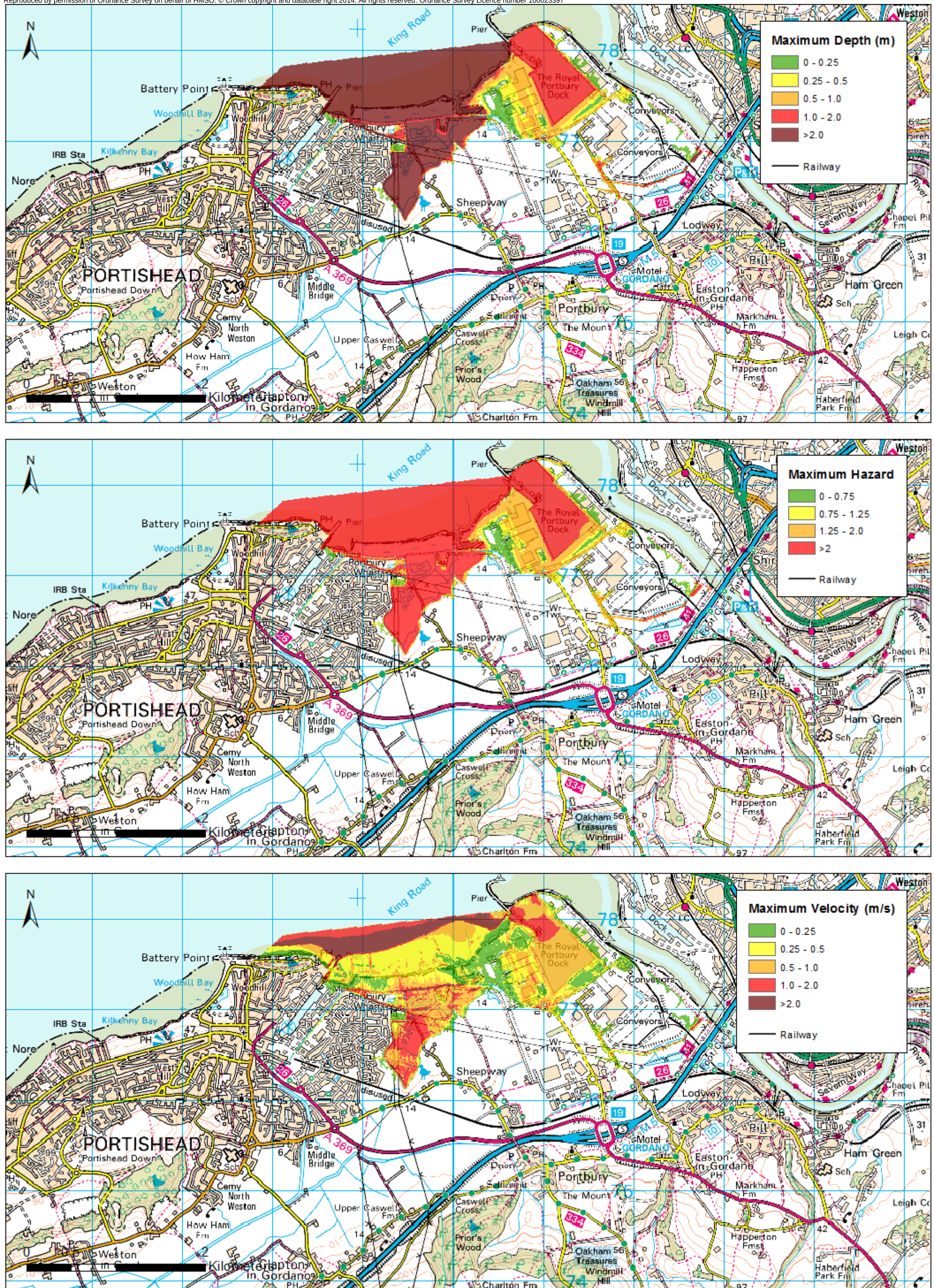
Figure M-3: Post Development Railway, 25 year return period - 2115
