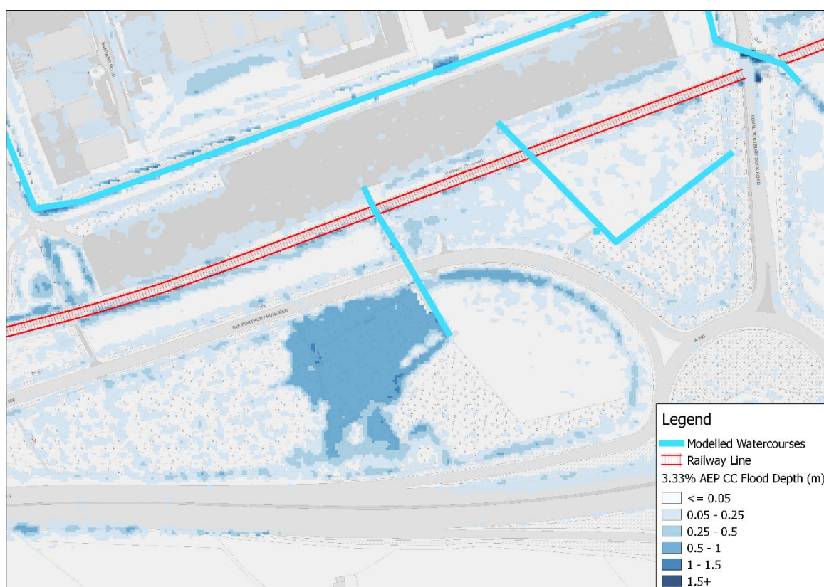
Figure K-10: Drove Rhyne 30 year return period, 2115 - 2
