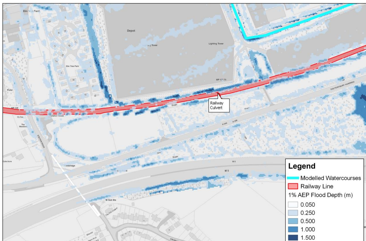
Figure K-3: Drove Rhyne 100 year return period- 1
