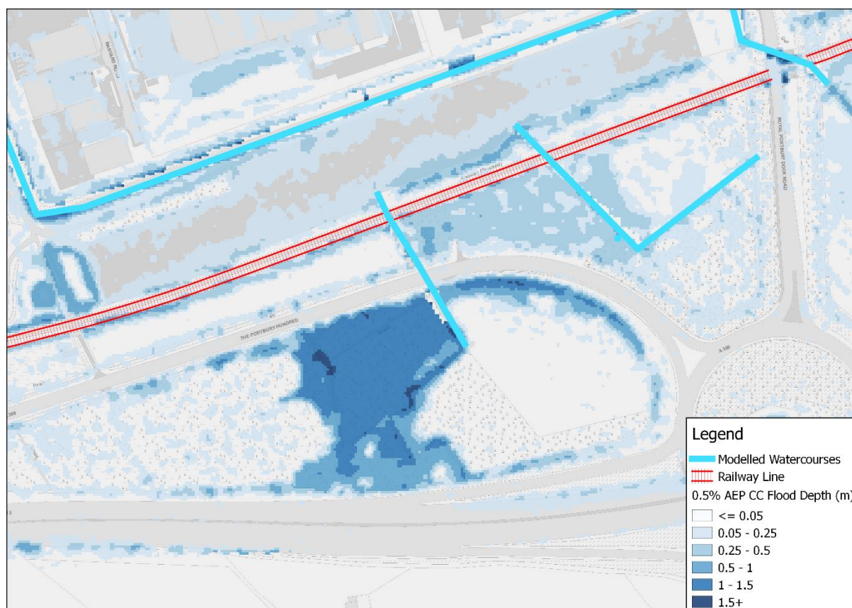
Figure K-14: Drove Rhyne 200 year return period, 2115 - 2
