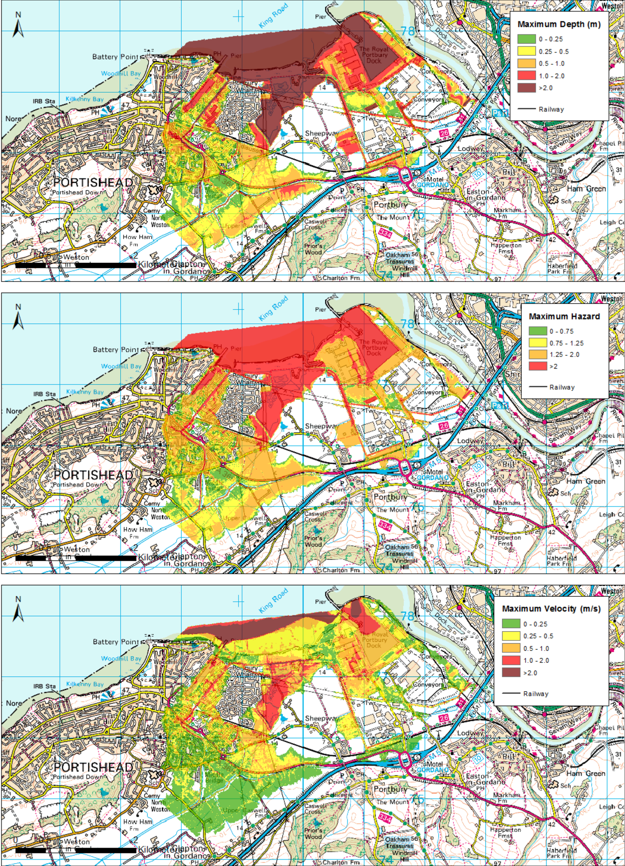
Figure M-12: Existing Railway, 1000 year return period - 2115
