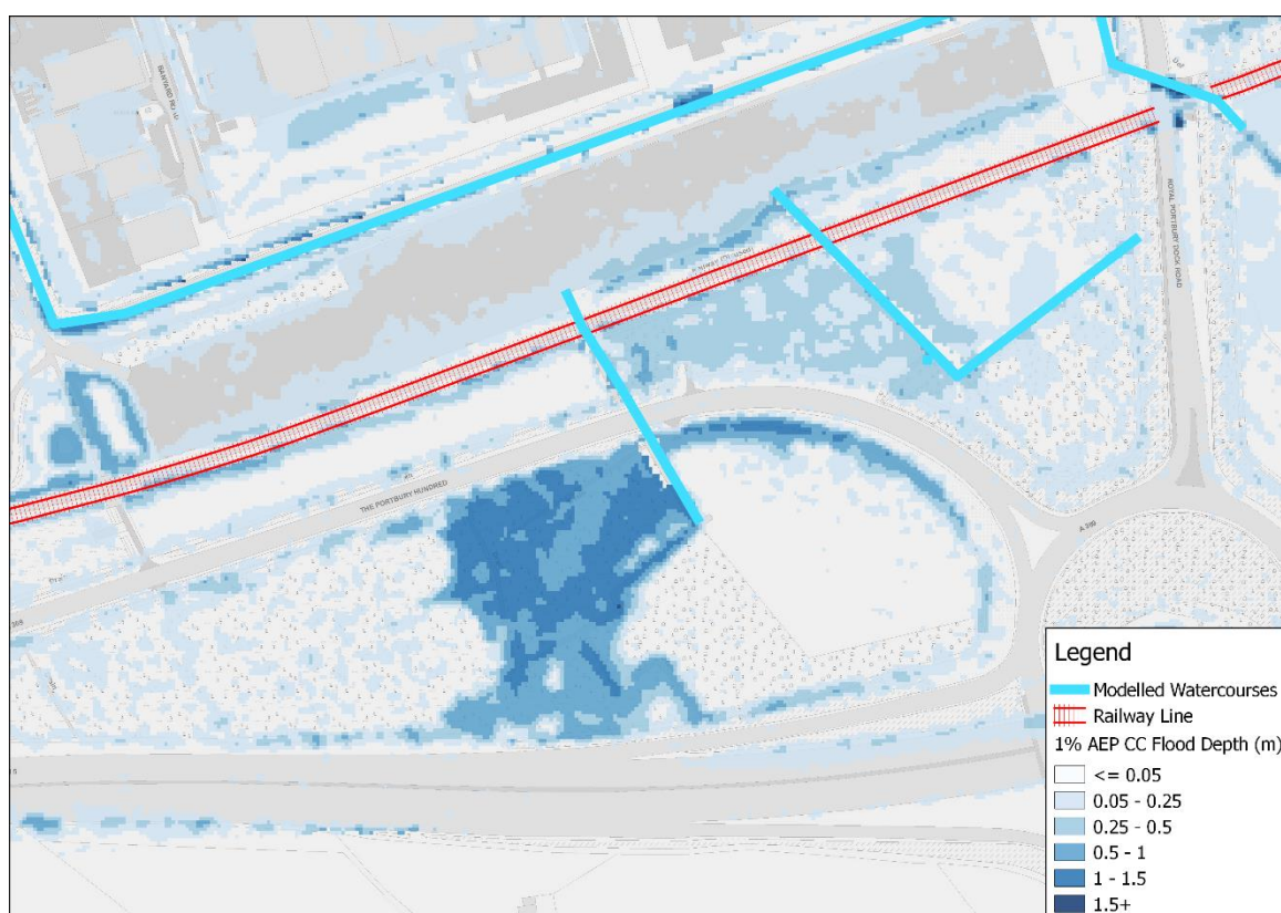
Figure K-12: Drove Rhyne 100 year return period, 2115 - 2
