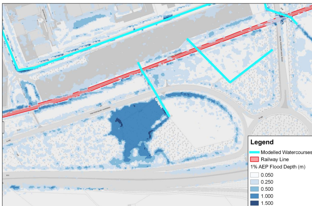
Figure K-4: Drove Rhyne 100 year return period- 2
