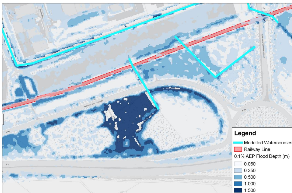
Figure K-8: Drove Rhyne 1000 year return period- 2
