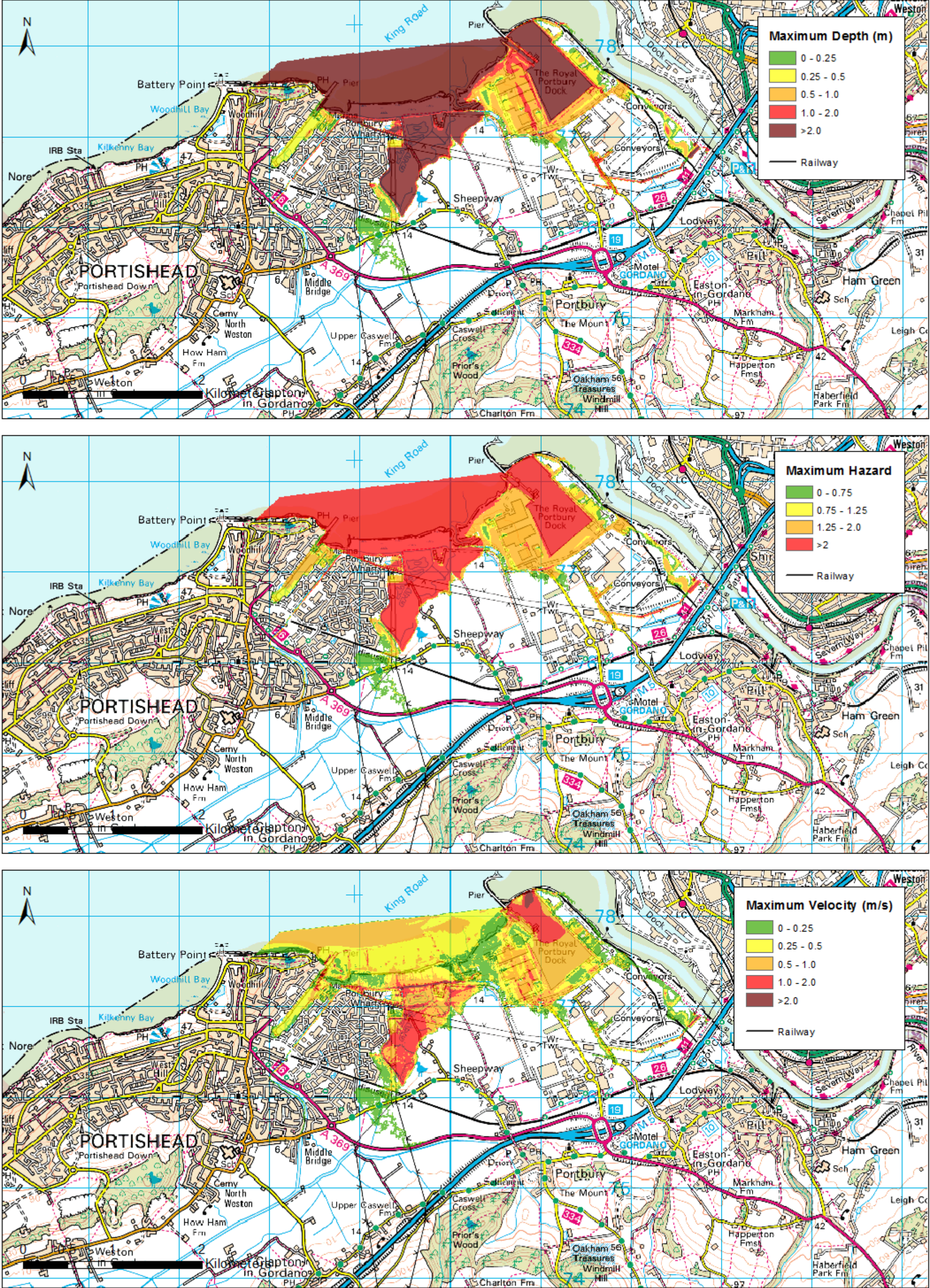
Figure M-9: Post Development Railway, 100 year return period - 2115
