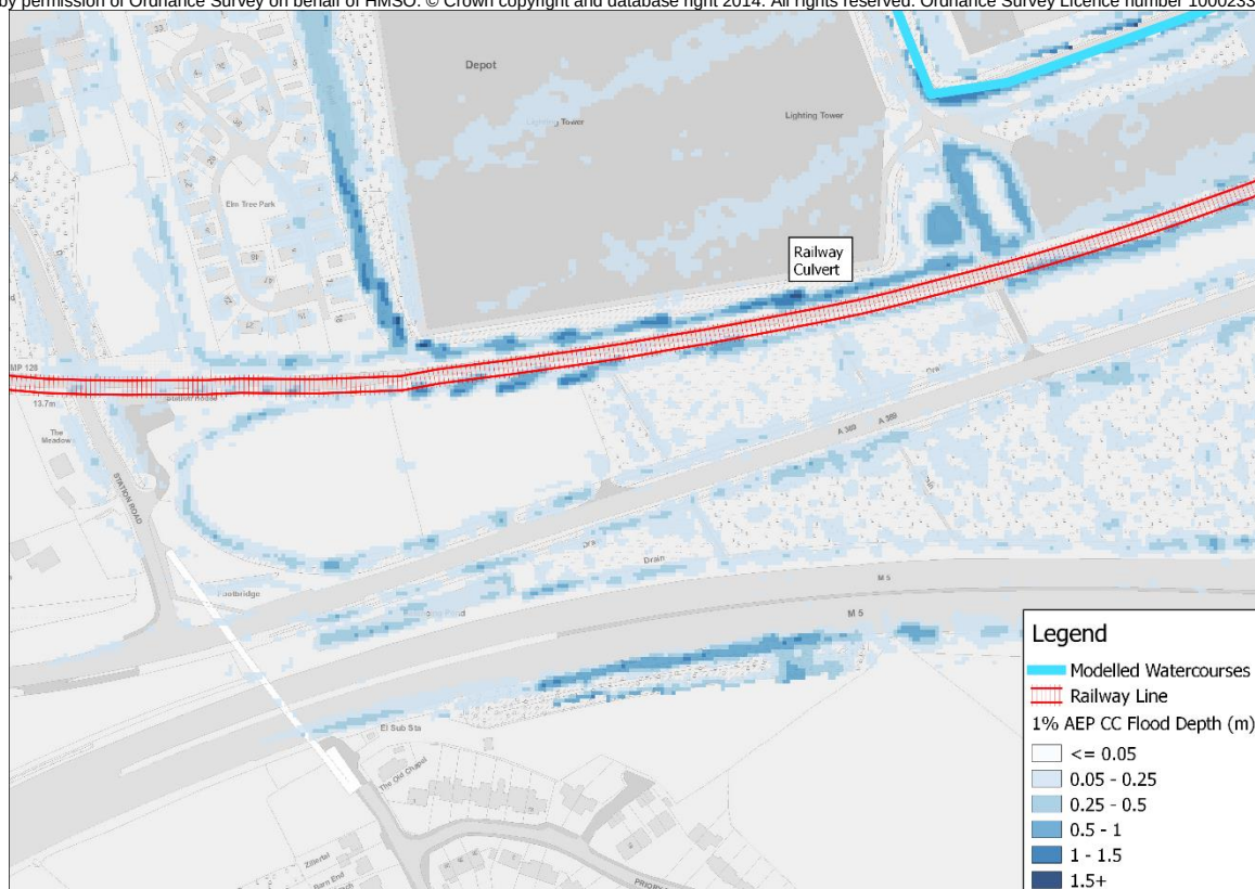
Figure K-11: Drove Rhyne 100 year return period, 2115 - 1
