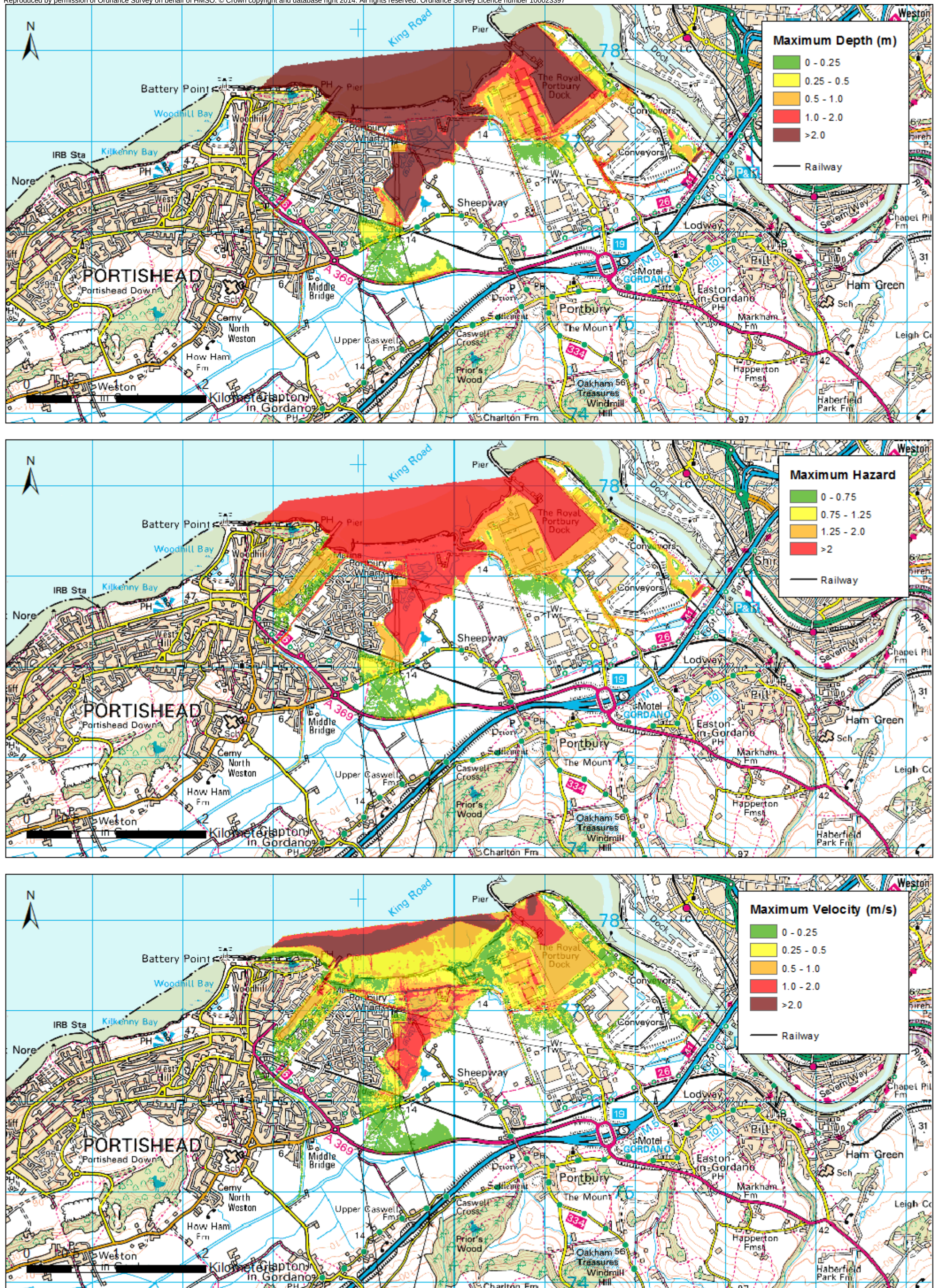
Figure M-10: Existing Railway, 200 year return period - 2115
