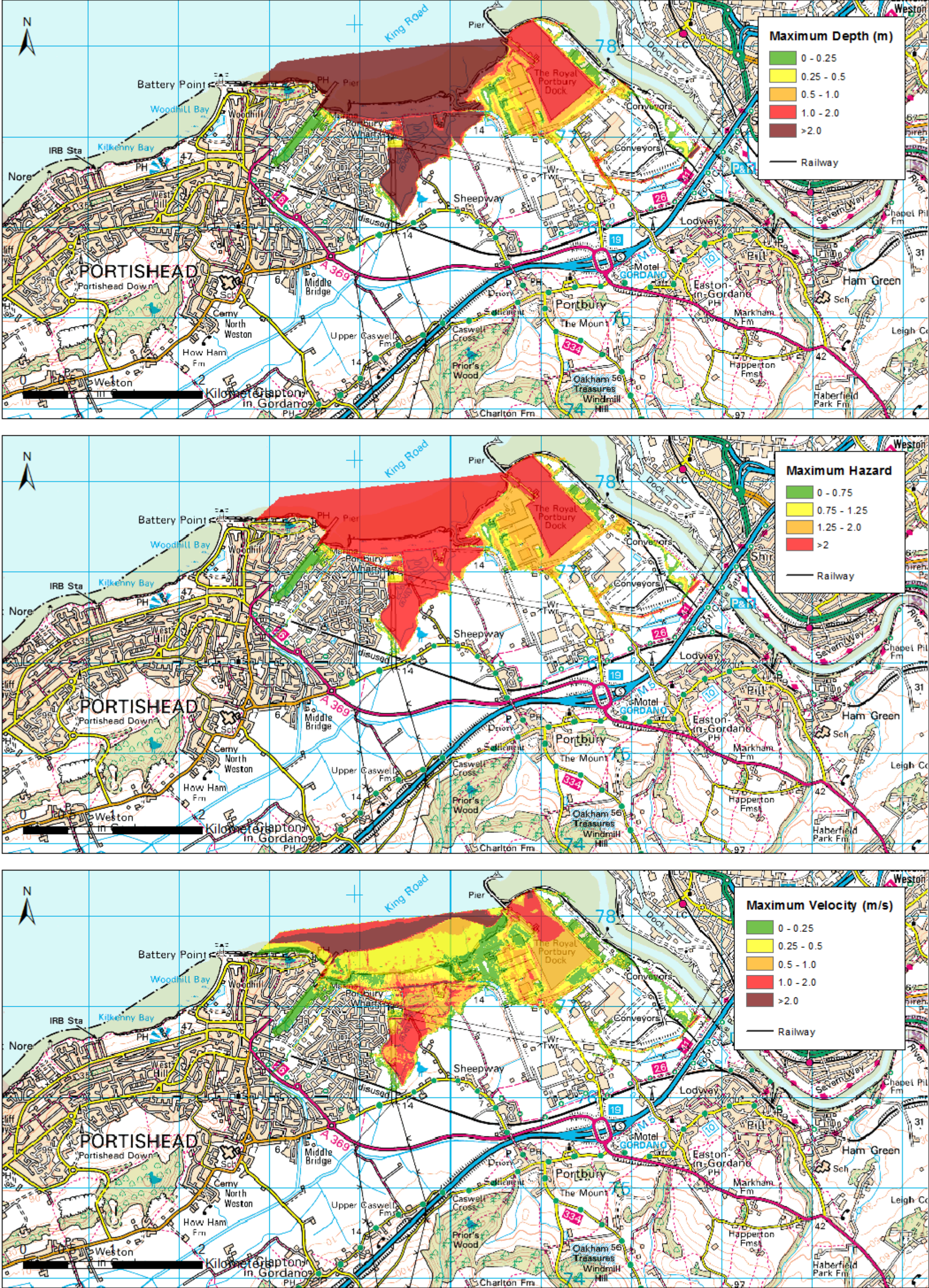
Figure M-5: Post Development Railway, 50 year return period - 2115
