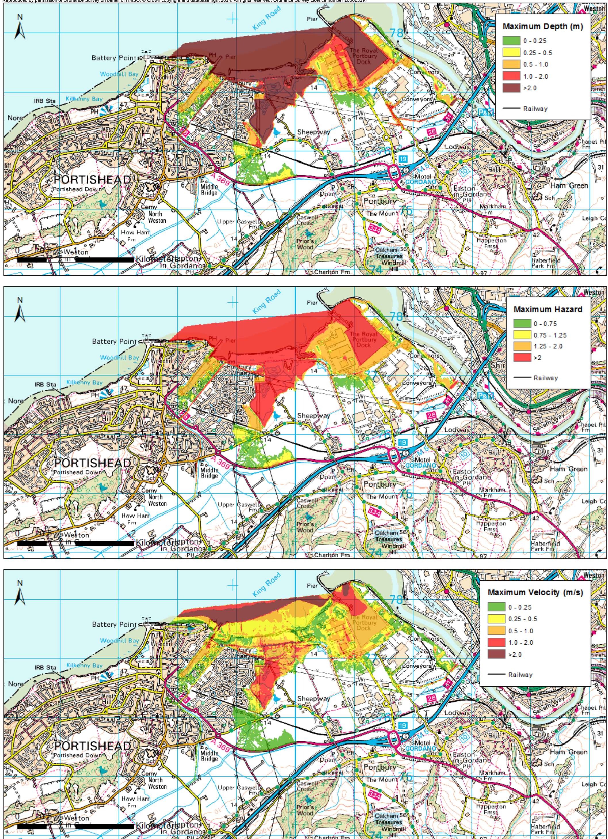
Figure M-11: Post Development Railway, 200 year return period - 2115
