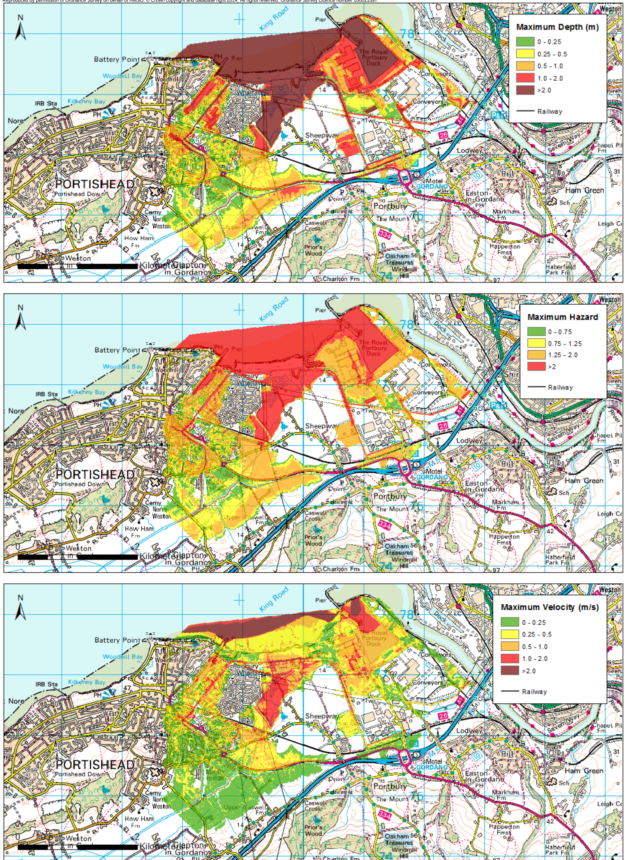
Figure M-13: Post Development Railway, 1000 year return period - 2115
